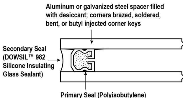
Figure 1: Dual-seal Type
